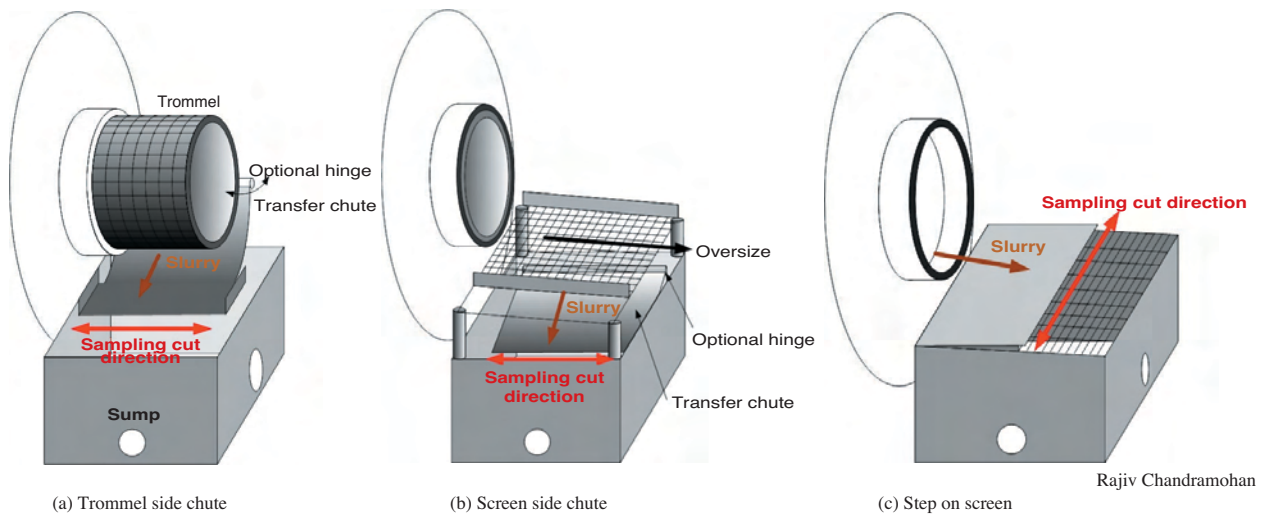
Figure 5—Mill discharge retrofit sample points
