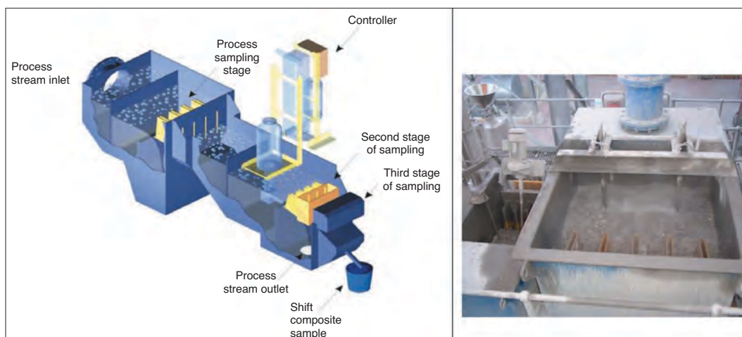
Figure 10—ANSTAT sampler
