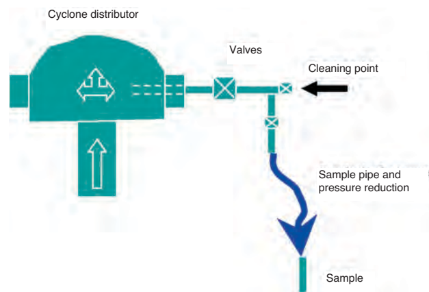
Figure 6—Cyclone feed probe sampler
