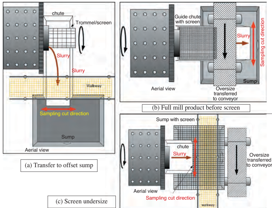
Figure 4—Mill discharge sampling
